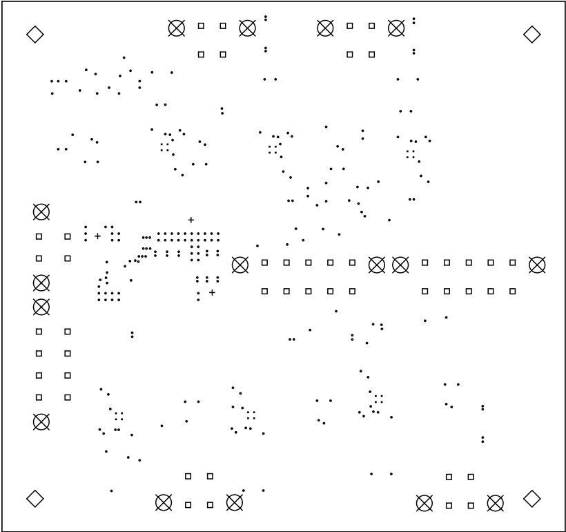
DRILL DRAWING SK-001-02 REV-A 08/05/2026
